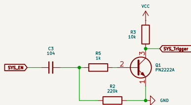
SYS Trigger/Reset
