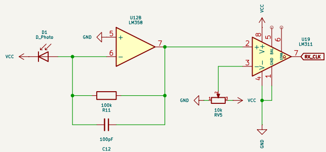
Optical Receiver Front-End
