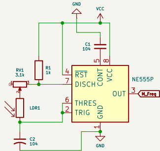
Frequency Generator
