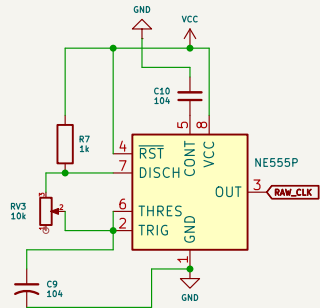
TX/RX System Clock
