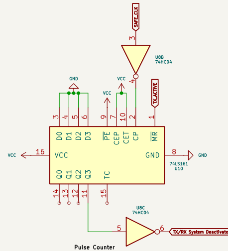
Pulse Counter
