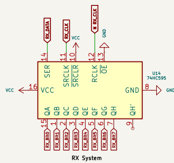
RX System
