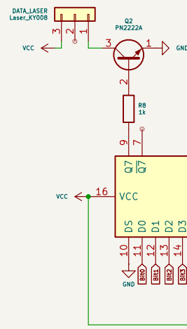
Pulse Counter
