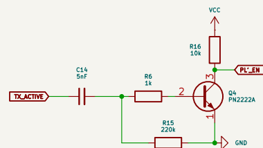
PL' Enable Signal
